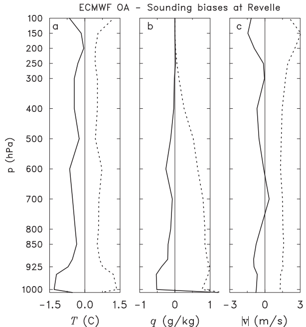
FIG. 2. Mean biases (solid) and rms differences (dashed) between ECMWF OA and soundings at R/V Reville for the period from 1 Oct to 31 Dec when the ship was at nominal location 0^\circ , 80.5^\circ\text{E} for (a) temperature, (b) specific humidity, and (c) wind speed.
